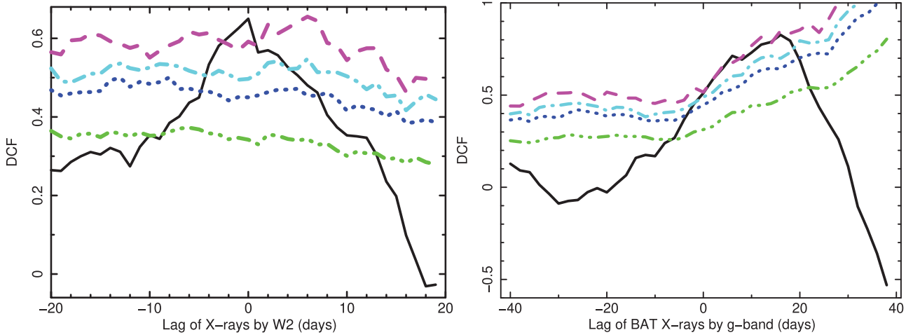
Figure 3. Left-hand Panel: Discrete cross-correlation function (DCF) between XRT (0.3–10 keV) and UVOT (UVW2) light curve . Green, Blue, cyan, and magenta line corresponding to 68, 90, 95, and 99 per cent confidence contours. Right-hand Panel: DCF computed with the smoothed light curves (averaged with a 10 d box-car filter) from BAT (15–50 keV) and g band .
