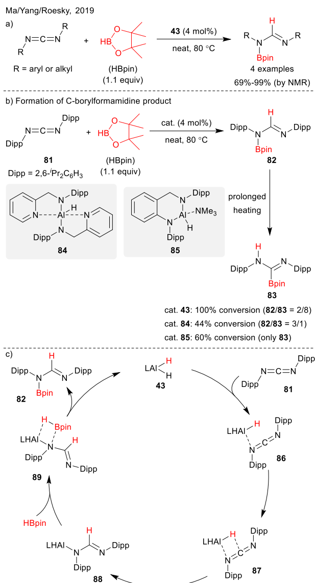
Scheme 21 N,N -bidentate ligated Al-complex catalysed hydroboration of carbodiimides.
