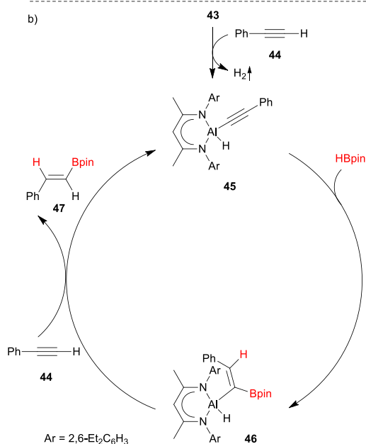
Scheme 10 \beta -diketimine ligated Al-complex catalysed hydroboration of alkynes.
