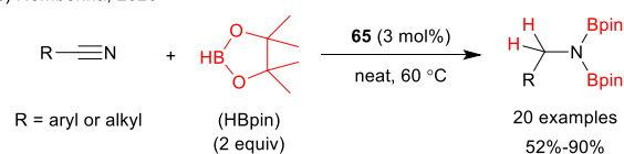
Scheme 20 a) and b) \beta -diketimine ligated Al-complex, c) CBG-supported Al-complex catalysed hydroboration of nitriles.
