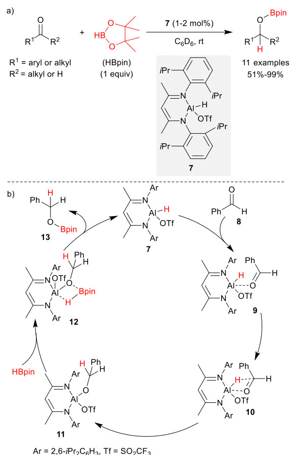
Scheme 4 β-diketimine ligated Al-complex catalysed hydroboration of carbonyl compounds.
