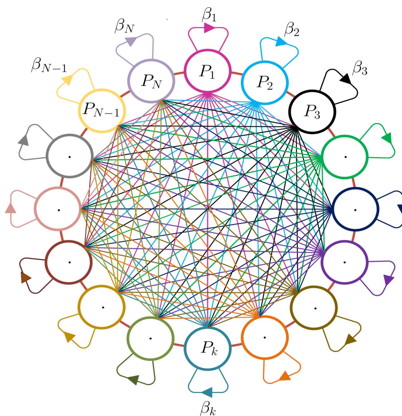
Figure 5: A schematic representation of N interacting population groups with different infection spread rates among each group. Every connection between two groups is bidirectional and symmetric, and every group is connected to all other groups (a dense network).
