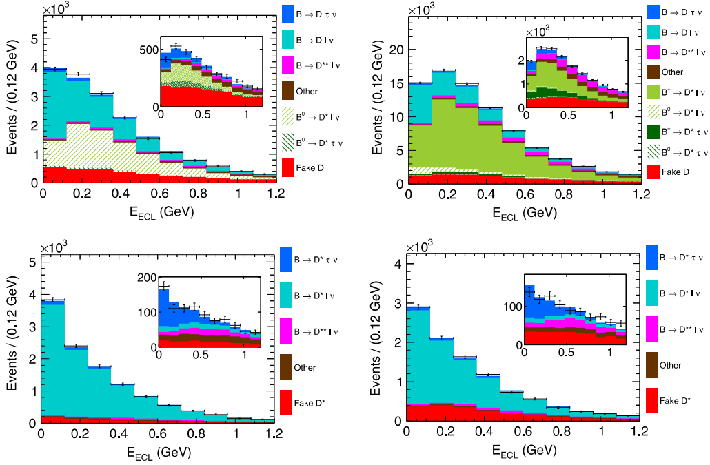
FIG. 1. E_{\text{ECL}} fit projections and data points with statistical uncertainties in the D^+ \ell^- (top left), D^0 \ell^- (top right), D^{*+} \ell^- (bottom left), and D^{*0} \ell^- (bottom right) samples, for the full classifier region. The signal region, defined by the selection O_{\text{cls}} > 0.9 , is shown in the inset with the same axis labels.
