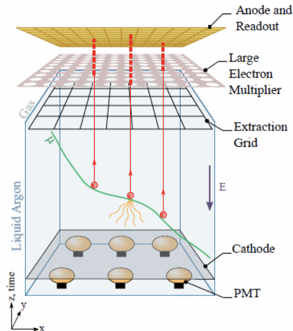
Figure 1.6: The general operating principle of the DP LArTPC. The ionization charges drift vertically upward in LAr and are transferred into a layer of argon gas above the liquid where they are amplified before collection on the anode. The light detectors (PMTs) sit under the cathode.
