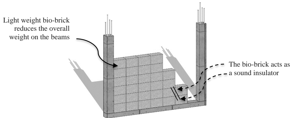
Figure 12. Filler wall material for column beam structure
