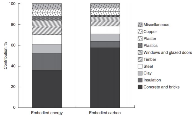
Figure 1. Constituent raw materials for building
