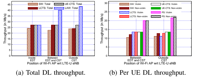
Fig. 13: Throughput results in Downlink only traffic for the three scenarios (i.e., inside EDT, between EDT and CST, and outside CST). LTE-U follows a 50% duty cycle with a period of 10ms, implying 5ms ON and OFF periods.
