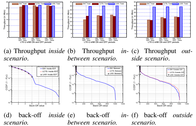
Fig. 14: Throughput and back-off of all three schemes.
