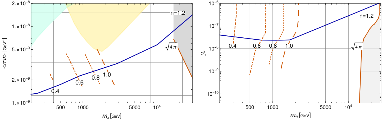
Fig. 3. The left and right panels show the allowed parameter space in the plane of (m_\chi, \langle\sigma v\rangle) and (m_N, y_N) , respectively. The observed relic density is obtained for the DM coupling \lambda = 0.4 (dashed), 0.6 (dot-dashed), 0.8 (dotted), 1.0 (long-dashed) and \sqrt{4\pi} (solid). The green and yellow shaded regions are excluded by Fermi-LAT (at 90% C.L.) and H.E.S.S. (at 95% C.L.) data, respectively. The blue solid curve represents future bound from CTA where the region above (below) will be excluded at 90% C.L. for left (right) panel. The gray region is forbidden by perturbativity limit. The masses of \chi, N, \phi are assumed to follow m_\chi = n m_N = 1/n m_\phi with n = 1.2, \kappa = 1 , and the RHN is assumed to decay equally to each lepton flavor.
