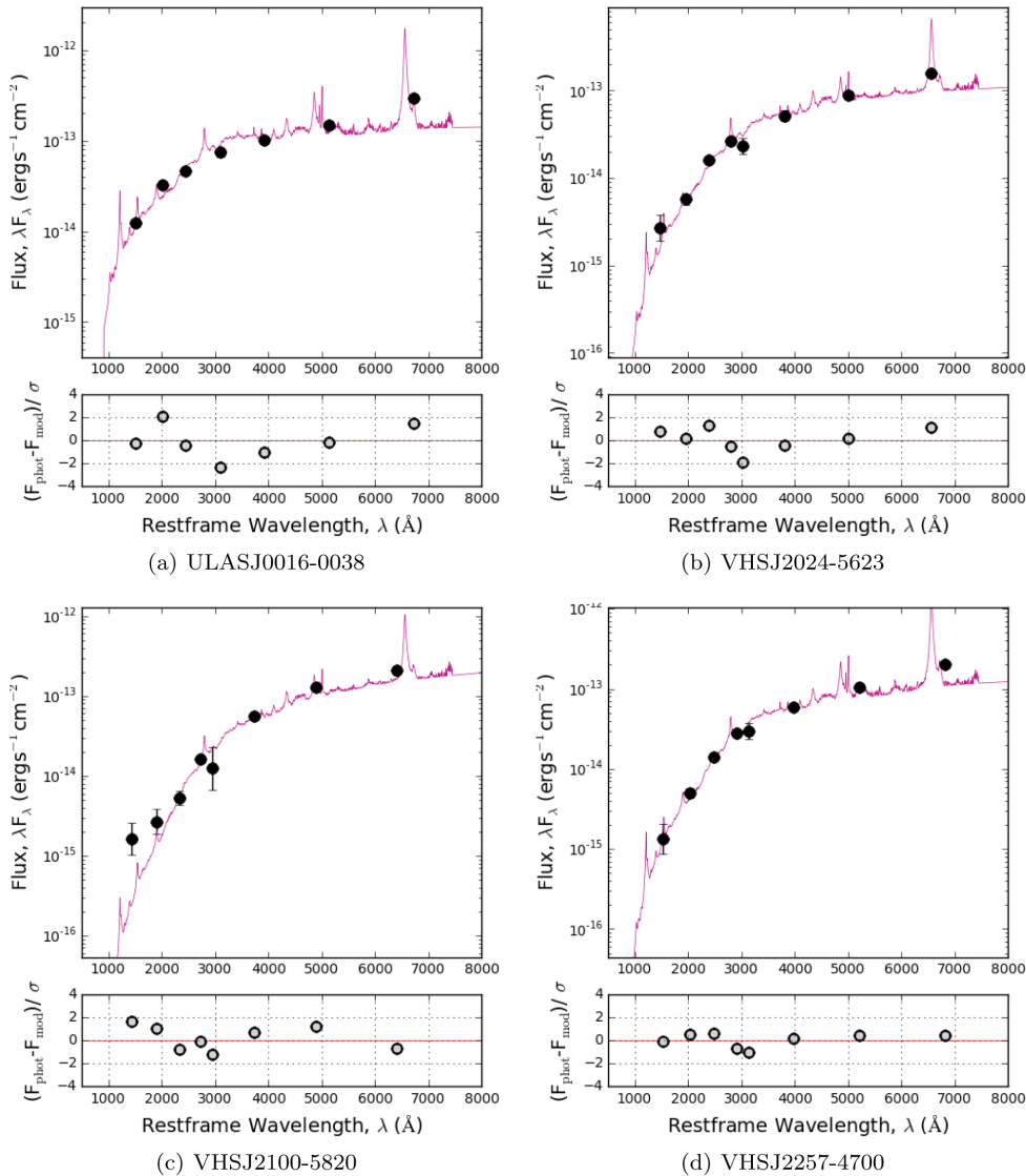
Figure 2. Upper panels: best-fitting quasar SEDs for ULASJ0016–0038 (a), VHSJ2024–5623 (b), VHSJ2100–5820 (c), VHSJ2257–4700 (d) for which \chi_{\text{red,QSO}}^2 < 2.5 . Black points show the griZ Y DES and JHK VHS/ULAS photometry. Lower panels: the error-weighted residuals for each fit.
