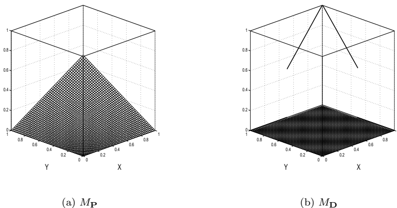
FIGURE 2. The conditionally cancellative (proper) t-subnorms M_{\mathbf{P}} and M_{\mathbf{D}} from Remark 4.3
