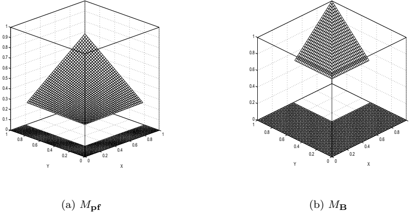
FIGURE 1. While M_{\mathbf{Pf}} is a conditionally cancellative t-subnorm, M_{\mathbf{B}} is not.
