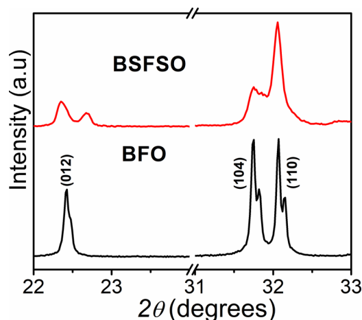
FIG. 2. XRD patterns of BFO and BSFSO compounds in the range 22^\circ \leq 2\theta \leq 32.7^\circ .
