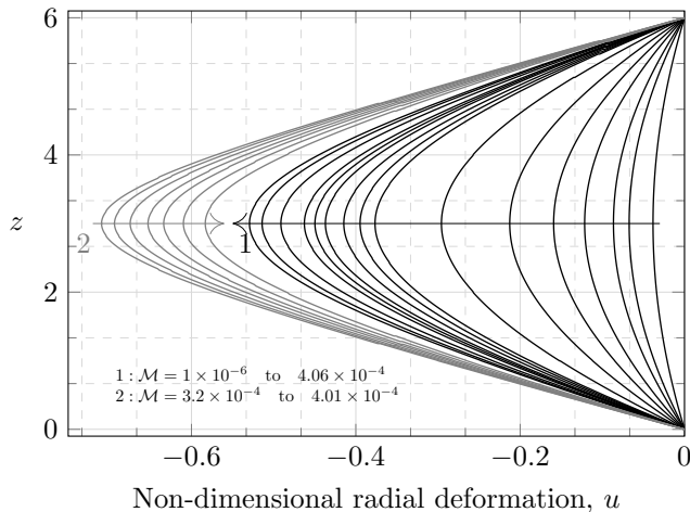
Figure 9: Deformation profiles of the cylindrical membrane under the influence of magnetic field alone ( P = 0 ). The arrows indicate the direction of increase in \mathcal{M} . Solutions from both the directions merge at the magnetic limit point and the corresponding value of the magnetic energy density parameter: \mathcal{M} \approx 4.07 \times 10^{-4} . This position moves away from the wire (located at u = -1 ) with increase in internal pressure. Not every value of \mathcal{M} has two corresponding stable solutions.
