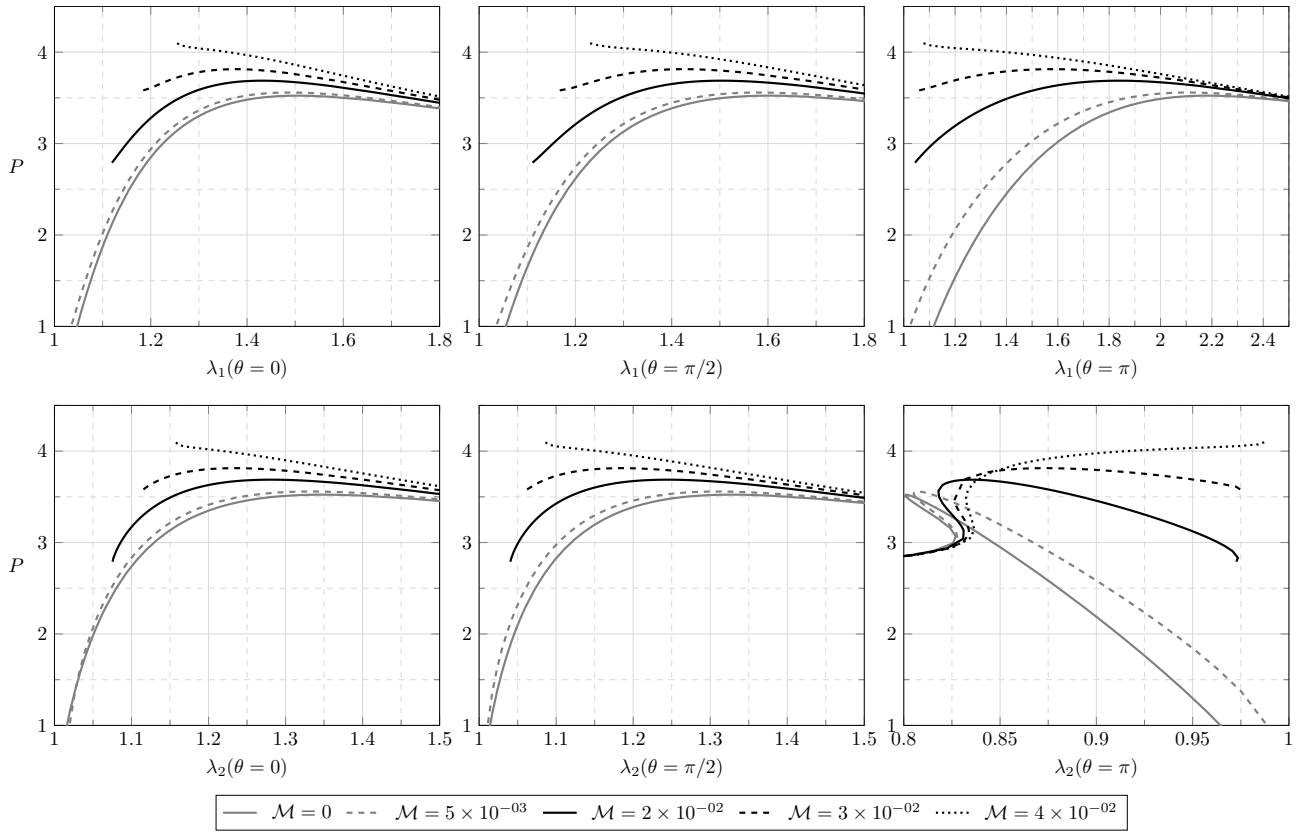
Figure 8: Variation of non-dimensional inflation pressure with principal stretches for initial radii of cross-section (a) r = 0.2 and (b) r = 0.5 . Note the behaviour of critical points with magnetic energy parameter \mathcal{M} and radius of cross-section r
