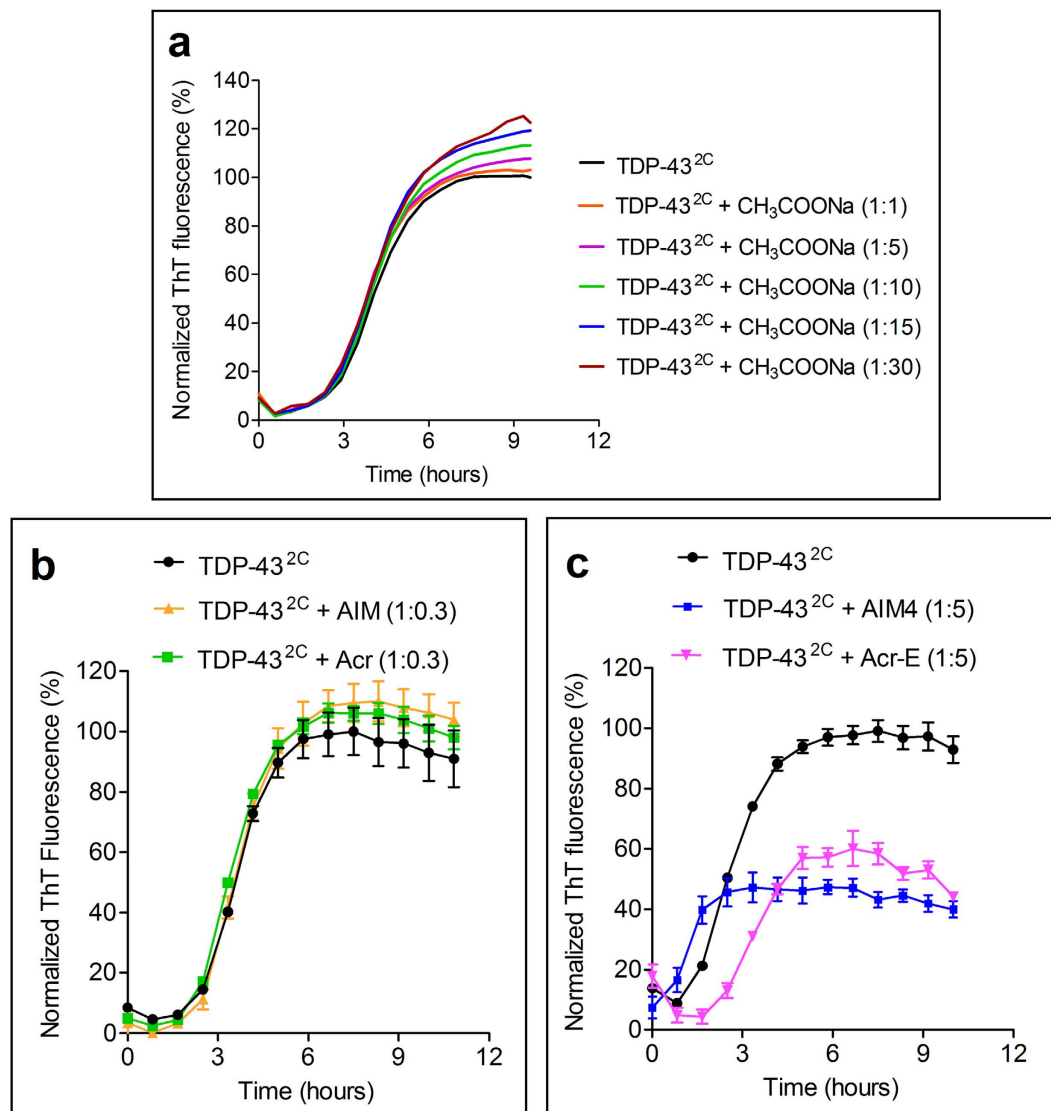
Figure 3. Effect of acetate ions & acridine derivatives on in vitro aggregation of TDP-43 2C . (a) TDP-43 2C (400 \mu M) solubilized in aggregation buffer was added with increasing concentrations of sodium acetate (1:1 to 1:30, protein: compound, molar ratio) that was also pre-dissolved in the aggregation buffer but lacking the Tris-HCl & DMSO. Aggregation trend was monitored by ThT fluorescence at 37 ^{\circ} C for 15 hours with intermittent agitation (15 seconds agitation every 5 minutes). Increasing stoichiometry of sodium acetate caused concomitant marginal increase in the overall ThT fluorescence. (b) Aggregation trend of TDP-43 2C in presence of Acr and AIM was monitored by ThT fluorescence. TDP-43 2C (400 \mu M) was added with 125 \mu M Acr or 125 \mu M AIM (protein: compound ratio of 1:0.3) in aggregation buffer lacking Tris-HCl and containing 8% DMSO final. The protein aggregation was examined at 37 ^{\circ} C for 15 hours with intermittent agitation by recording ThT fluorescence intensity. A sample lacking any compound was incubated similarly for comparison. (c) TDP-43 2C aggregation in presence of Acr-E was monitored by recording ThT fluorescence intensity. TDP-43 2C (400 \mu M) was added with 2000 \mu M Acr-E or in the control experiment with 2000 \mu M AIM4, in aggregation buffer containing 12 mM Tris-HCl and 8% DMSO final. Samples were incubated at 37 ^{\circ} C for 15 hours with intermittent agitation and ThT fluorescence was recorded. A sample lacking any compound was incubated & monitored similarly for comparison. Acr-E and AIM4 were found to respectively reduce the ThT fluorescence by 45% and 55%.
