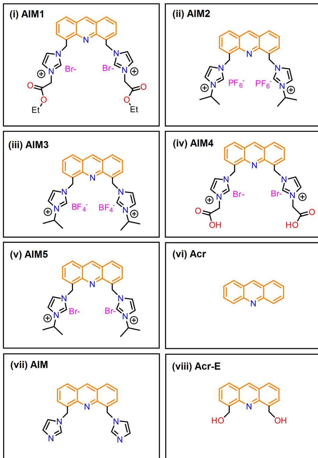
Figure 1. Structures of acridine derivatives examined for effect on TDP-43 2C aggregation. AIM1: [4,5-bis((N-ethoxycarbonyl methyl imidazolium)methyl)acridine] dibromide; AIM2: [4,5-bis((N-isopropylimidazolium) methyl) acridine] hexafluorophosphate; AIM3: [4,5-bis((N-isopropylimidazolium) methyl)acridine] tetrafluoroborate; AIM4: [4,5-bis((N-carboxy methyl imidazolium)methyl)acridine] dibromide; AIM5: [4,5-bis((N-isopropylimidazolium) methyl) acridine] dibromide; Acr: Acridine; AIM: (4,5-bis(imidazole methyl)acridine) and Acr-E: (4,5-bis(hydroxymethyl)acridine).
