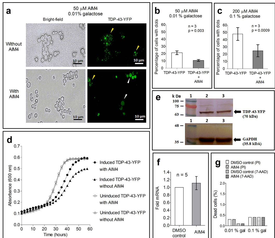
Figure 6. Inhibition of TDP-43-YFP aggregation by AIM4 in yeast model. (a) Fluorescence images of wild-type human TDP-43 tagged with YFP in the absence and presence of 50 \mu M AIM4 in S. cerevisiae strain with erg6 \Delta mutation after 4 hours of induction with 0.01% galactose. Formation of fluorescent foci (yellow arrows) indicates TDP-43-YFP aggregation while diffused fluorescence (white arrows) indicates the absence of TDP-43-YFP aggregation. (b) Percentage of TDP-43-YFP containing erg6 \Delta yeast cells displaying fluorescent dots in the absence or presence of AIM4 after 4 hours induction with 0.01% galactose. Error bars represent standard deviations ( p = 0.003 , n = 3 ; two-tailed t-test). (c) Percentage of TDP-43-YFP containing erg6 \Delta yeast cells displaying fluorescent dots in absence or presence of AIM4 after 4 hours induction of expression with 0.1% galactose. Error bars represent standard deviations ( p = 0.0009 , n = 3 ; two-tailed t-test). (d) Growth curve of TDP-43-YFP plasmid containing erg6 \Delta yeast cells cultured in SRaf-Ura media either under induced (0.1% galactose) or un-induced state which were either treated or not treated with 200 \mu M AIM4. Data from triplicate cultures were averaged. (e) Effect of AIM4 (200 \mu M) on TDP-43-YFP protein expression levels in S. cerevisiae erg6 \Delta cells determined by western blotting using anti-GFP antibody. Protein bands of TDP-43 YFP and the protein loading control, endogenously expressed GAPDH (probed with anti-GAPDH antibody) have been cropped from the original image (Supplementary Fig. S2). Similar TDP-43-YFP levels were observed in absence (Lane 2) or presence (Lane 3) of AIM4. (f) Effect of AIM4 on TDP-43-YFP mRNA levels determined by Real-Time PCR. Expression of TDP-43-YFP was induced (0.01% galactose, 4 hours) either in presence of 200 \mu M AIM4 or DMSO buffer (control). Actin was used as the endogenous control. No significant change in TDP-43-YFP mRNA levels was observed. The error bar indicates standard deviation from five independent samples ( n = 5 ). Cytotoxicity of AIM4 (200 \mu M) on erg6 \Delta yeast cells analyzed by propidium iodide (PI) and 7-aminoactinomycin D (7-AAD) staining using flow cytometry (total: 50,000 cells) using PE-Texas Red-A & PerCP-Cy5-5A filters respectively. Similar percentage of dead cells indicate lack of AIM4 cytotoxicity at this concentration.
