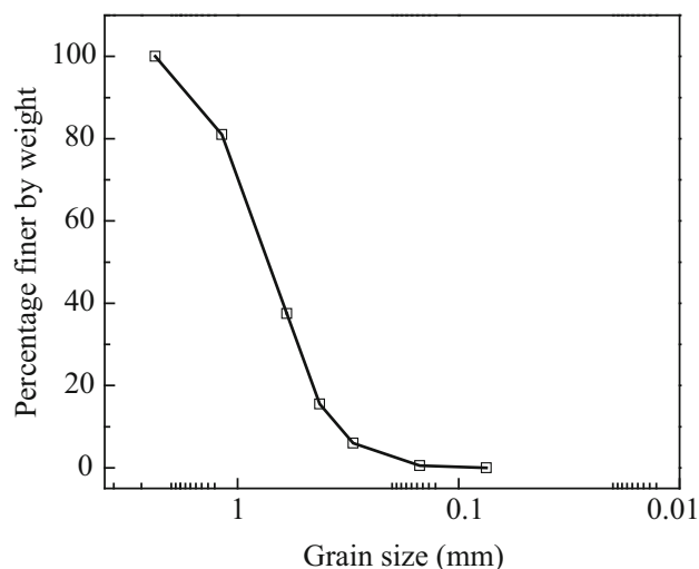
Fig. 1 Grain-size distribution curve of sand
