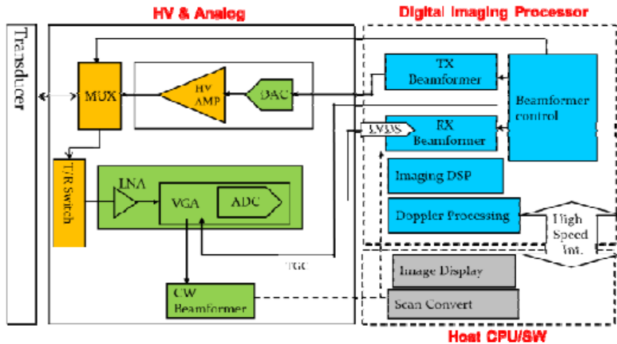
Fig. 7.1 Medical Ultrasound imaging system [26]
