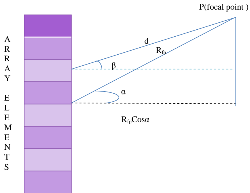
Fig 5.1 Distance calculation in dual angle architecture
