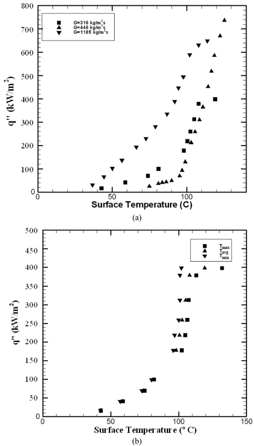
Figure 7. Boiling curve for 65 micron channel with (a) different mass flux values and (b) G = 316 kg/m 2 s with maximum, minimum and average temperatures.
