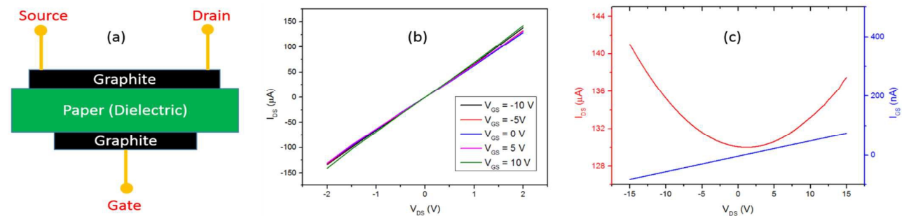
Figure 2: (a) Schematic diagram of all graphite paper field effect transistor; (b) output characteristics of FET; (c) transfer characteristics of FET showing drain current (Red) and leakage current (Blue).
