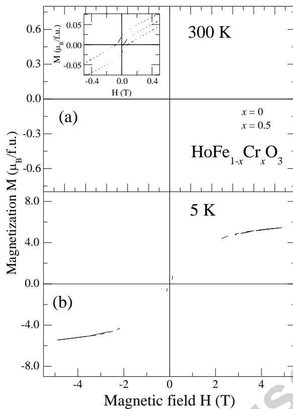
Fig. 3: Magnetic field vs. Magnetization graph for \text{HoFe}_{1-x}\text{Cr}_x\text{O}_3 ( x = 0, 0.5 ) compounds (a) at 300 K. Inset shows the expanded view for x = 0 compound (b) Magnetization graphs at 5 K for x = 0 and x = 0.5 compounds respectively.
