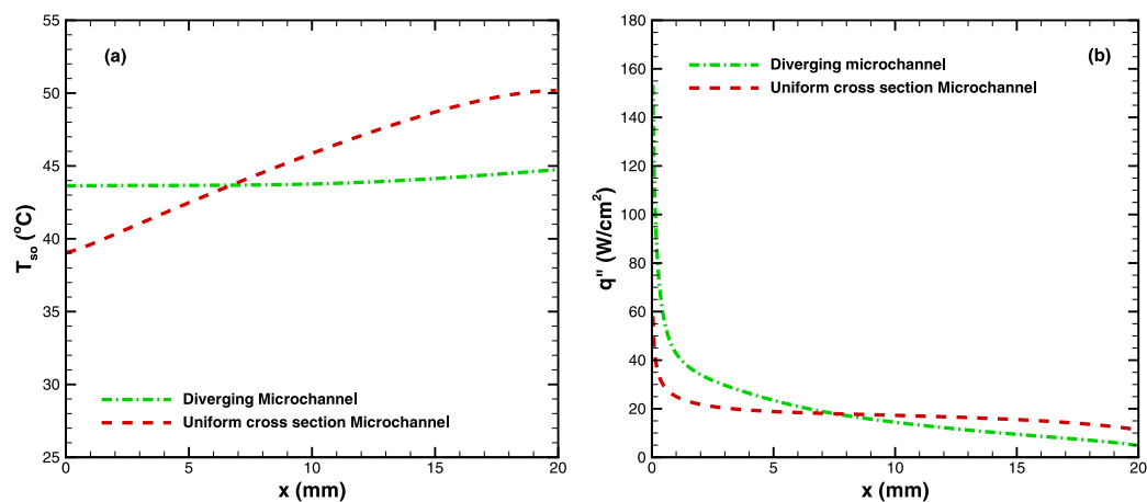
Figure 2. Comparison of (a) surface temperature, (b) heat flux distribution in a diverging and a straight microchannel obtained numerically.
