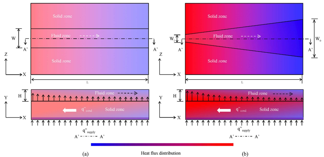
Figure 1. Schematic representation of proposed method to bring constant wall temperature condition (a) Uniform cross section microchannel, (b) Diverging microchannel.
