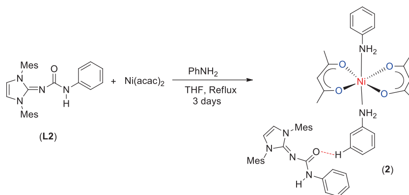
Scheme 2. Synthesis of nickel complex 2 .
