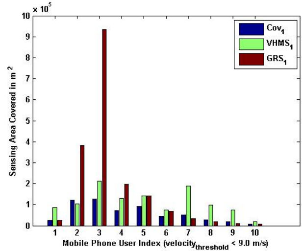
Fig. 12. Sensing Area Covered
