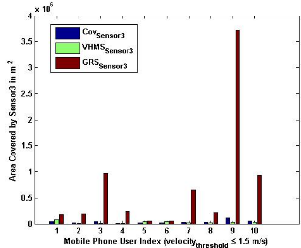
Fig. 16. Sensing Area Covered by Sensor3
