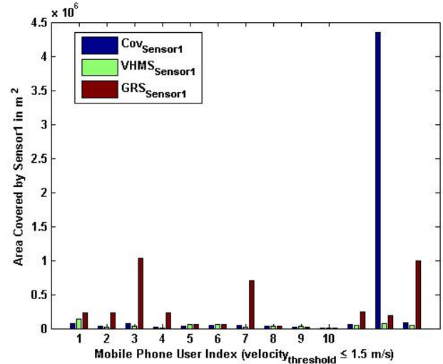
Fig. 14. Sensing Area Covered by Sensor1
