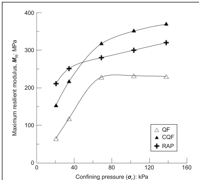
Figure 3. Variation of maximum resilient moduli with confining pressure
