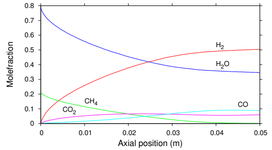
Figure 12: Species mole fraction along reactor length. Inlet conditions for reforming channel and oxidation channel are given in Table 1
