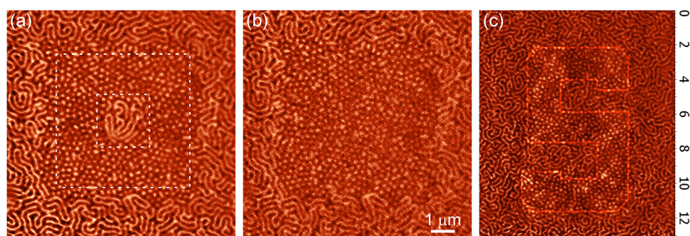
Figure 4. Zero-field MFM images of the domain structure of the (Pt/CoFeSiB/W) 11 with the created area filled by skyrmions and with non-scanned central region (a). The outer and inner borders indicated by white dashed lines delimit the scanning region in the tapping mode. The same area after full filling by skyrmions (b). Realization of the S symbol by skyrmion nanolithography on the surface of the (Pt/CoFeSiB/W) 11 film (c). The MFM image size is 11 \times 13 \mu\text{m}^2 . The red line delimits the tapping mode scanned area.
