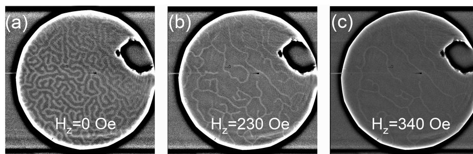
Figure 1. MTXM images of the domain structure of the (\text{Pt}/\text{CoFeSiB}/\text{W})_{11} sample captured at zero field (a), H_z = 230 Oe (b), and H_z = 340 Oe (c). The diameter of the viewing area is 10\ \mu\text{m} .
