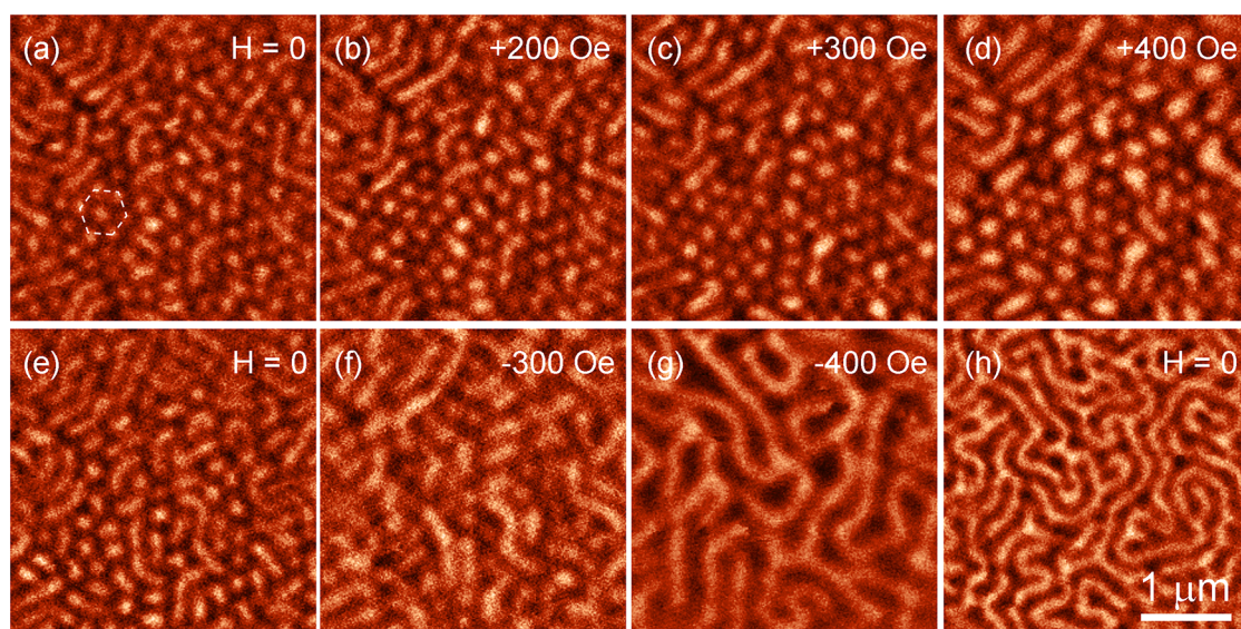
Figure 2. MFM images of the domain structure of the (Pt/CoFeSiB/W) 11 film recorded after the five-pass scanning in the tapping mode in the fields from 0 to +400 Oe (a–d), then from 0 to –400 Oe (e–g), and again in zero field (h). The dashed line in (a) marks a hexagonal unit cell of the skyrmion lattice. The bright contrast corresponds to the magnetization oriented along the positive external field, and the dark one corresponds to the magnetization oriented along the negative direction.
