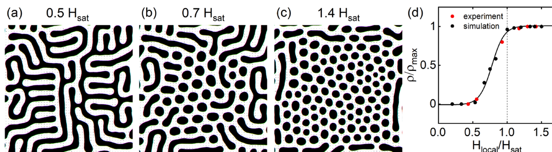
Figure 7. (a–c) Simulated domain structure of the (Pt/CoFeSiB/W) 11 film after the five-pass scanning with different local field values ( H_{\text{local}} ) expressed in units of the saturation field ( H_{\text{sat}} ). (d) Dependence of the normalized density of the skyrmions on the H_{\text{local}}/H_{\text{sat}} ratio.
