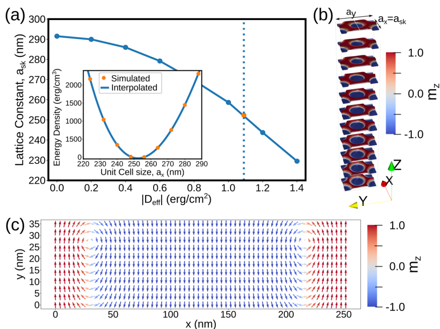
Figure 8. (a) Skyrmion lattice constant as a function of the IDMI strength. The vertical dashed line indicates the value of D_{\text{eff}} = -1.09 \text{ erg/cm}^2 measured experimentally. The inset presents the method of calculation of the lattice constant for D_{\text{eff}} = -1.09 \text{ erg/cm}^2 , i.e., minimization of the energy density as a function of the lattice constant. (b) The hexagonal skyrmion lattice simulated by a centered rectangular unit cell for D_{\text{eff}} = -1.09 \text{ erg/cm}^2 . (c) The XZ -plane at the Y center of the unit cell with a color scale proportional to the m_z magnetization component.
