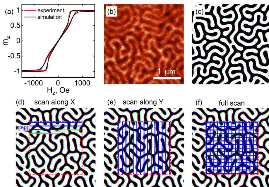
Figure 6. (a) Experimental and simulated out-of-plane hysteresis loops for the (Pt/CoFeSiB/W) 11 film. Domain structure at remanence captured by MFM (b) and generated by simulations (c). Schemes of the tip scanning trajectories in the micromagnetic simulations: (d) X direction, (e) Y direction, and (f) after the X and Y scans.
