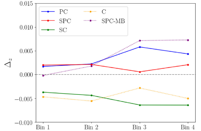
Figure 8. Mean redshift difference \Delta_z in each tomographic bin for each redshift sample being tested: SPC, SC, PC, SPC-MB, C, relative to the average mean redshift of SPC, SC, and PC. Spectroscopic catalogues are labelled as S, the PAUS+COSMOS catalogue as P, and the COSMOS2015 as C. SPC, SC, and PC (solid lines) are the three redshift samples used in this work. SPC-MB shows the effect of extrapolating the bias between S and C to all galaxies that are still using redshift information from C in SPC (mainly faint galaxies) (see Section 3.3 for a definition of the different samples used in this figure). The mean redshift is obtained by computing the n(z) from SOMPZ using each sample.
